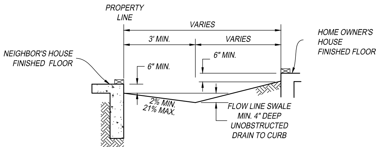
TYPICAL DRAINAGE DETAIL
